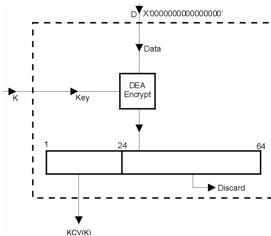
Figure 31 - Single-length Key Check Value KCV(K).
